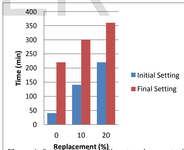
Figure 4. Setting time for different replacement of water hyacinth
