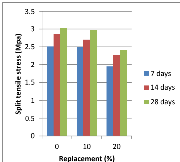
Figure 6. Split tensile Stress for different replacement of water hyacinth
